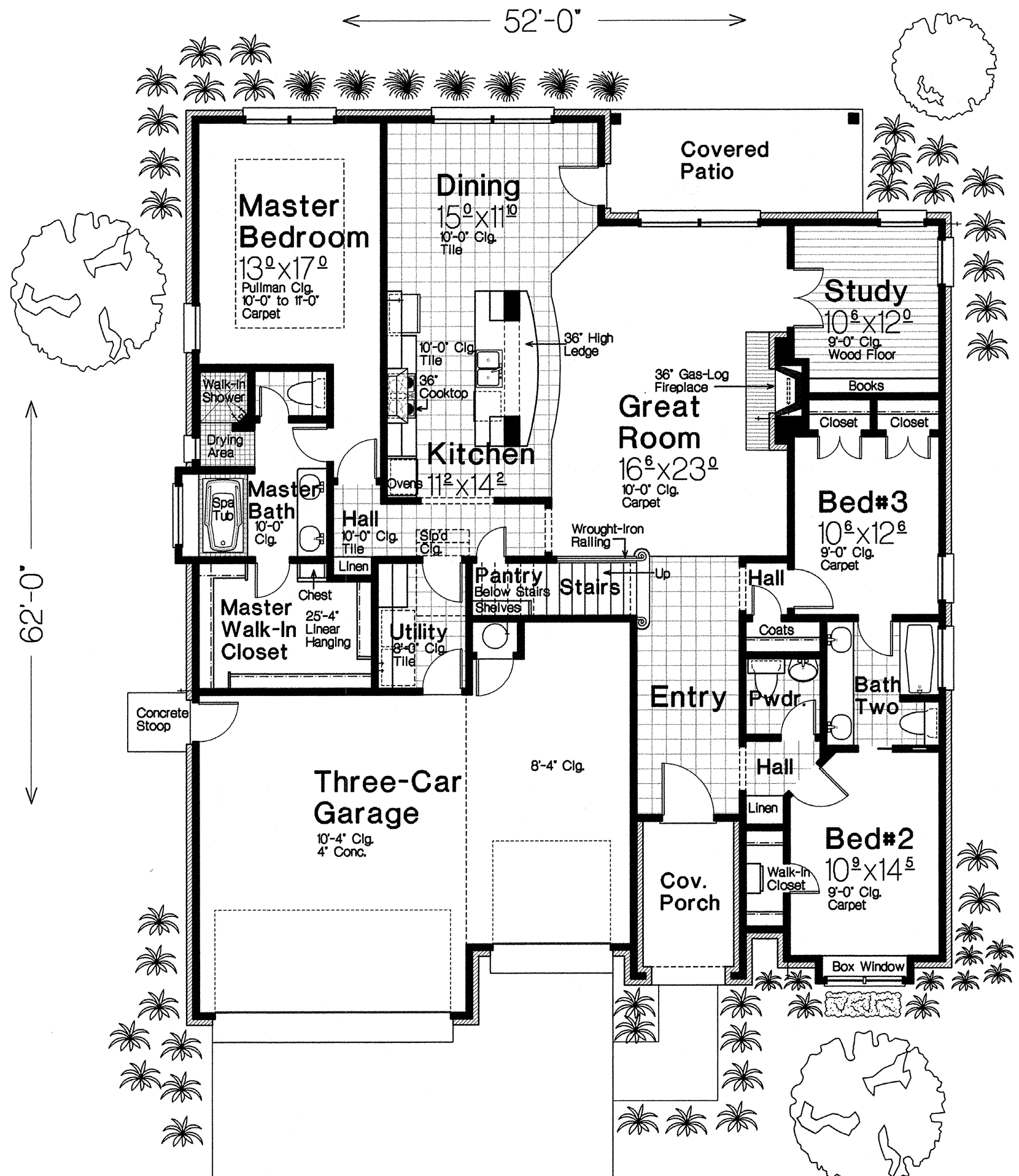
Main Floor 2170 Sq. Ft. Total ( Heated & Cooled ) Areas only First Floor Only PLAN NO. F2257 All Ceiling Heights 9'-0" & 10'-0" Unless Noted. Future Recreation Room Not Included in Total Sq. Ft.
